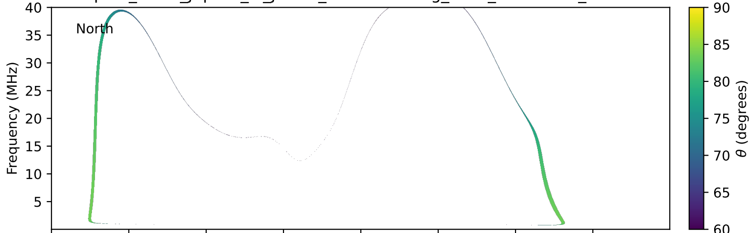
expres_earth_jupiter_io_jrm33_lossc-wid1deg_3kev_20130509_v11.cdf
