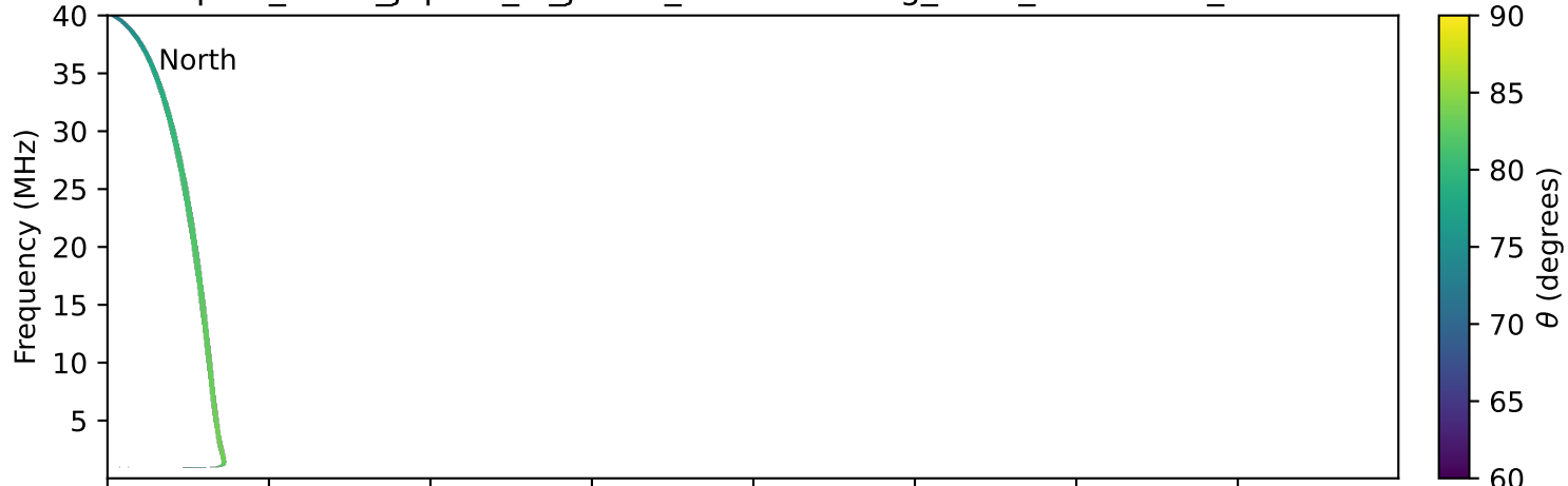
expres_earth_jupiter_io_jrm33_lossc-wid1deg_3kev_20130508_v11.cdf
