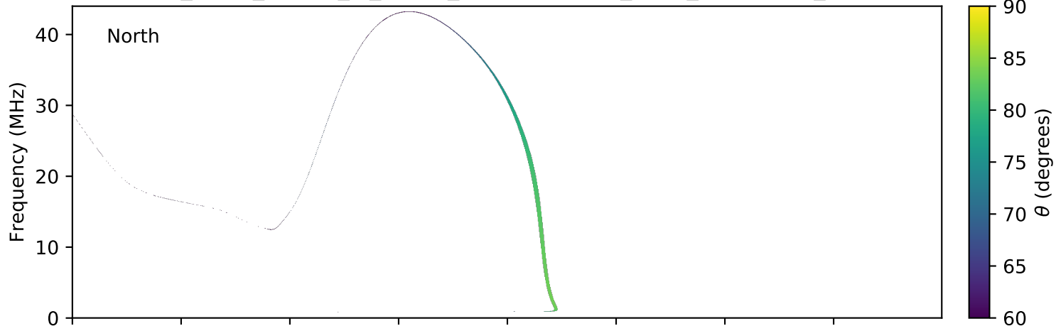
expres_earth_jupiter_io_jrm09_lossc-wid1deg_3kev_20130527_v01.cdf
