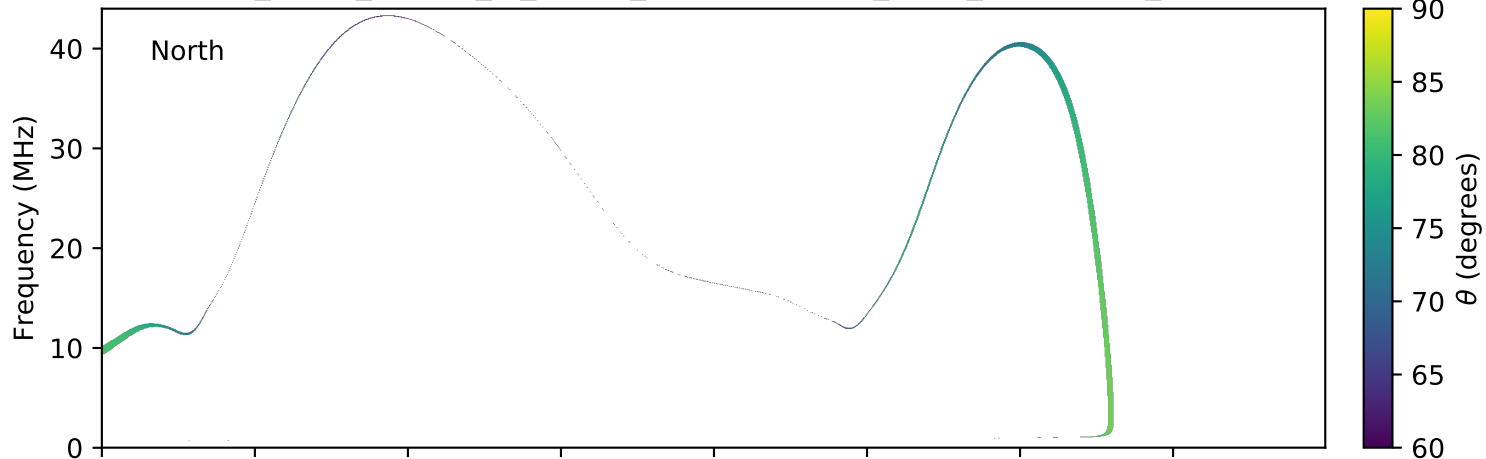
expres_earth_jupiter_io_jrm09_lossc-wid1deg_3kev_20130525_v01.cdf
