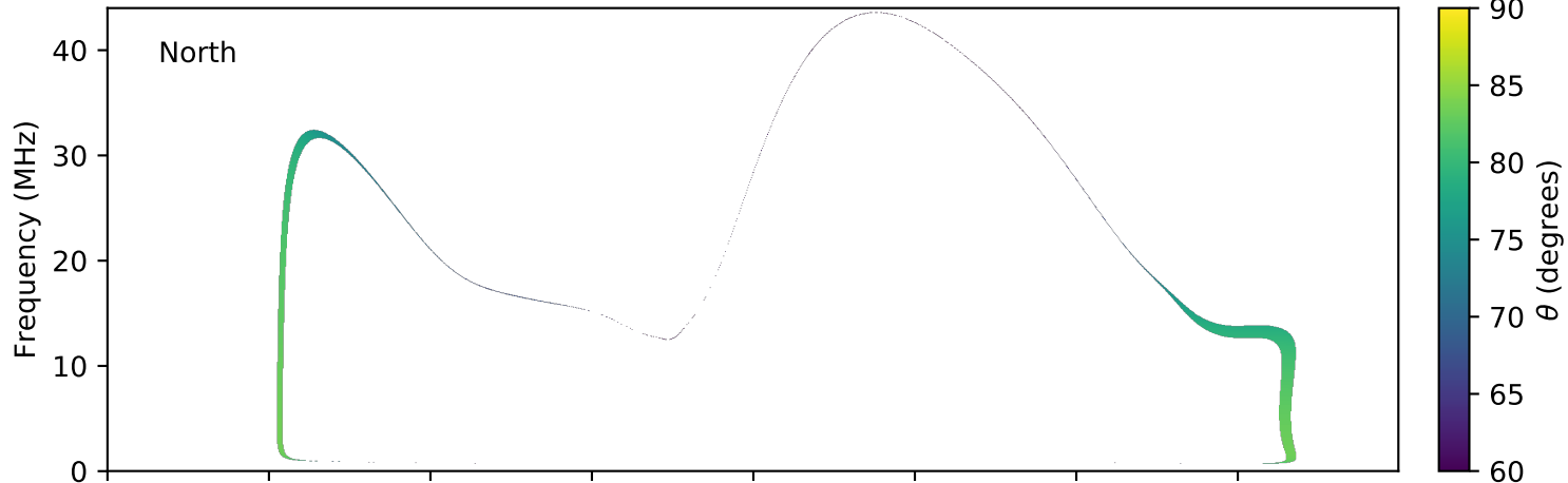
expres_earth_jupiter_io_jrm09_lossc-wid1deg_3kev_20130516_v01.cdf
