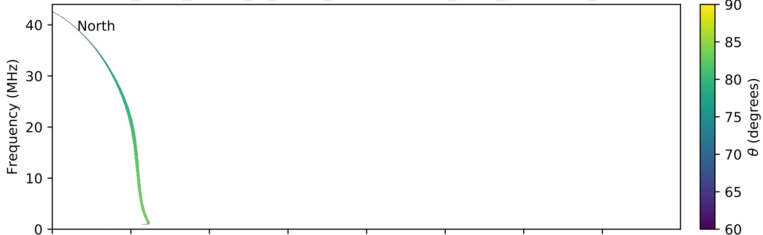
expres_earth_jupiter_io_jrm09_lossc-wid1deg_3kev_20130515_v01.cdf
