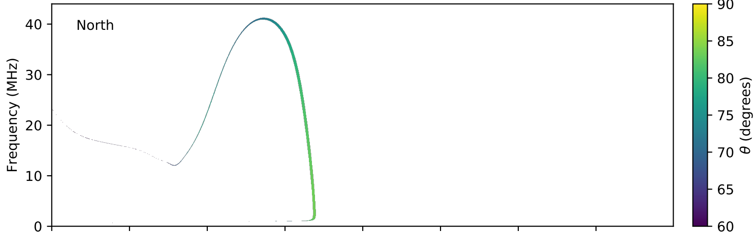
expres_earth_jupiter_io_jrm09_lossc-wid1deg_3kev_20130513_v01.cdf
