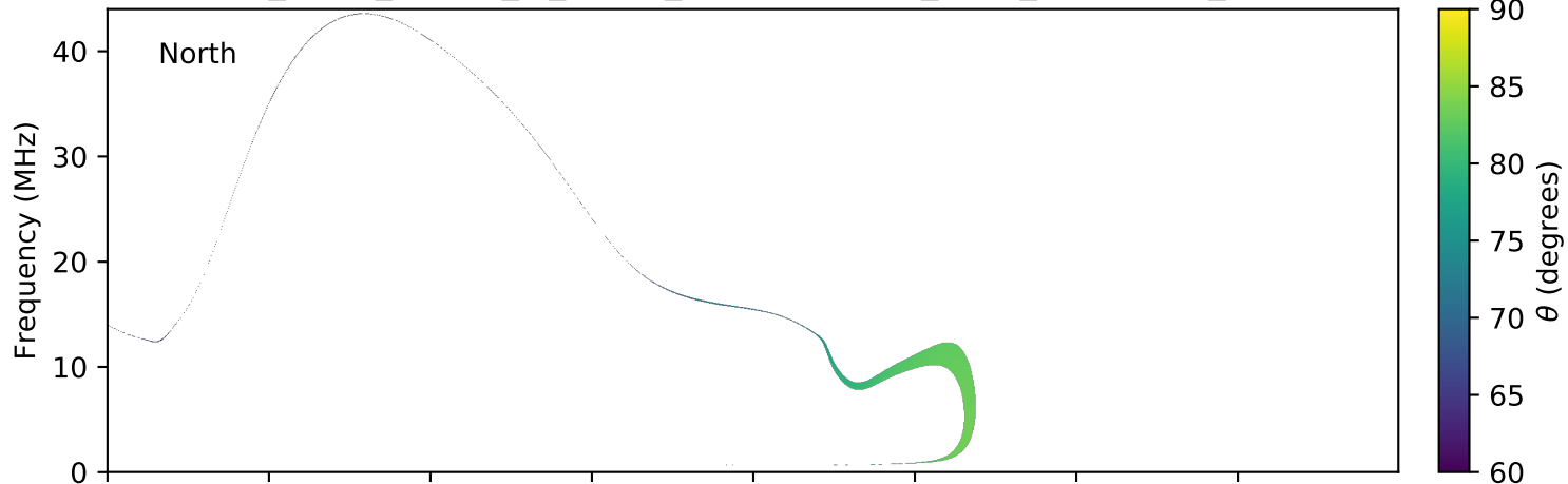
expres_earth_jupiter_io_jrm09_lossc-wid1deg_3kev_20130511_v01.cdf
