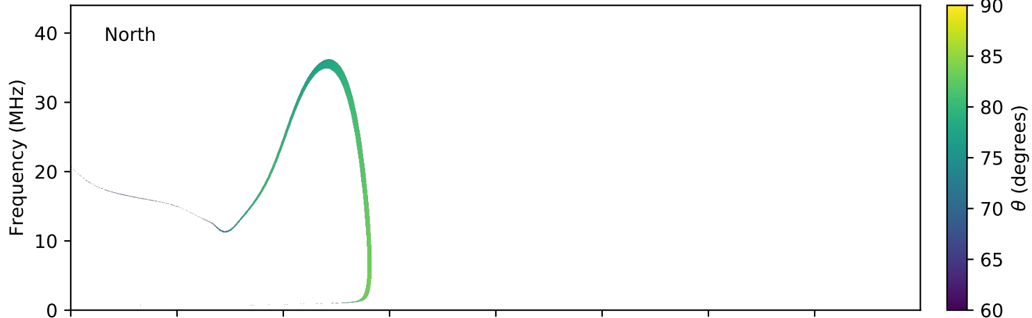
expres_earth_jupiter_io_jrm09_lossc-wid1deg_3kev_20130506_v01.cdf
