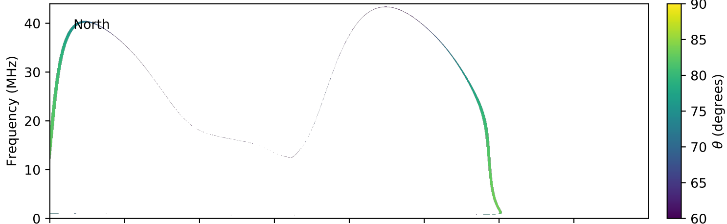
expres_earth_jupiter_io_jrm09_lossc-wid1deg_3kev_20130502_v01.cdf
