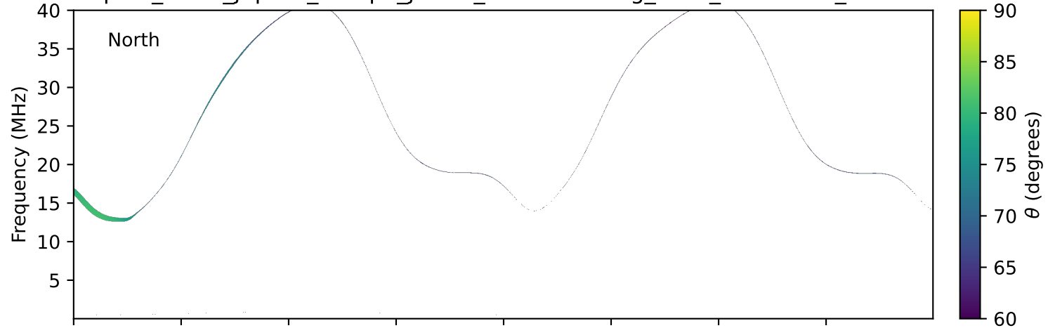
expres_earth_jupiter_europa_jrm33_lossc-wid1deg_3kev_20130501_v11.cdf
