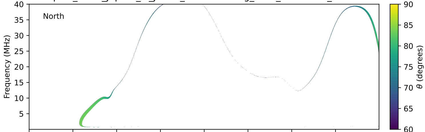
expres_earth_jupiter_io_jrm33_lossc-wid1deg_3kev_20130430_v11.cdf
