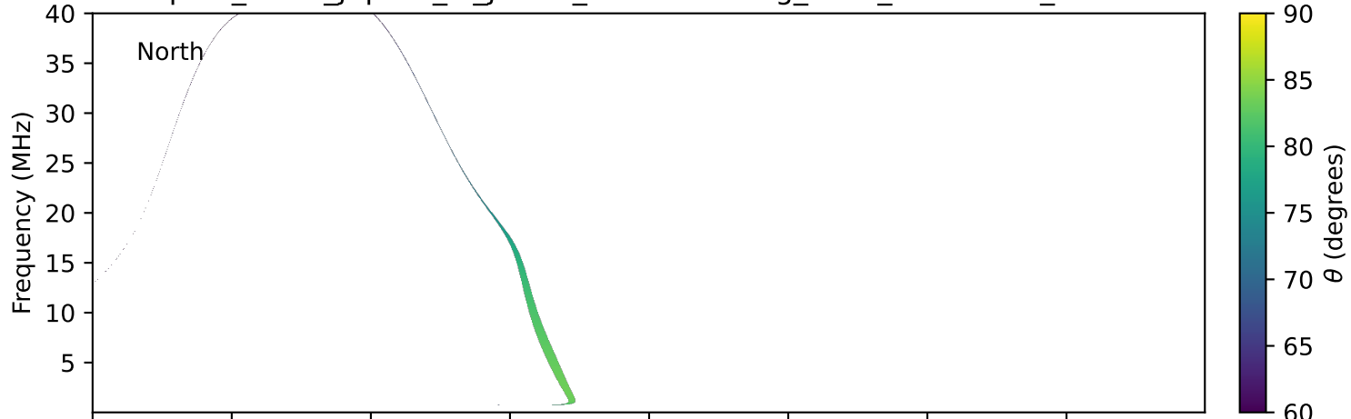
expres_earth_jupiter_io_jrm33_lossc-wid1deg_3kev_20130427_v11.cdf
