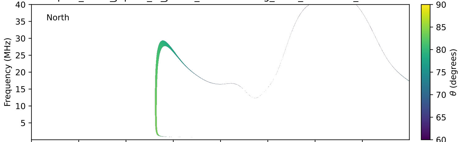
expres_earth_jupiter_io_jrm33_lossc-wid1deg_3kev_20130421_v11.cdf
