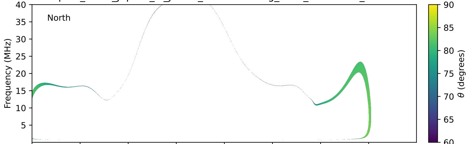
expres_earth_jupiter_io_jrm33_lossc-wid1deg_3kev_20130416_v11.cdf
