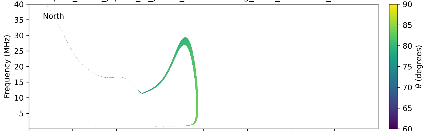
expres_earth_jupiter_io_jrm33_lossc-wid1deg_3kev_20130404_v11.cdf
