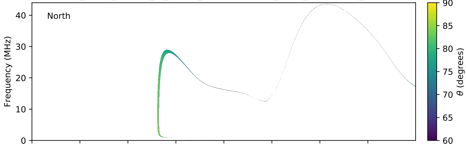
expres_earth_jupiter_io_jrm09_lossc-wid1deg_3kev_20130421_v01.cdf
