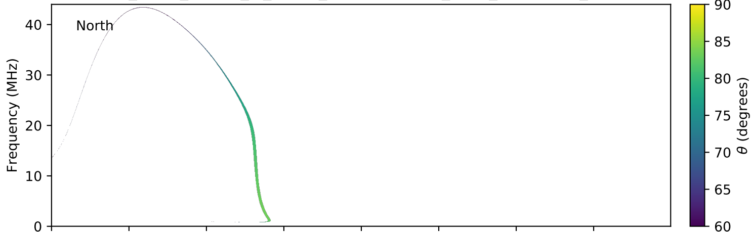
expres_earth_jupiter_io_jrm09_lossc-wid1deg_3kev_20130420_v01.cdf
