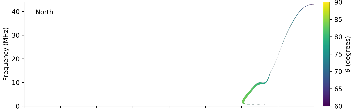
expres_earth_jupiter_io_jrm09_lossc-wid1deg_3kev_20130417_v01.cdf
