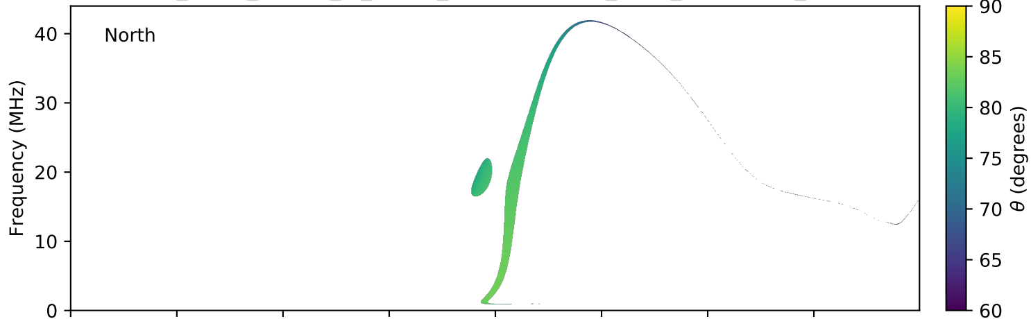
expres_earth_jupiter_io_jrm09_lossc-wid1deg_3kev_20130412_v01.cdf
