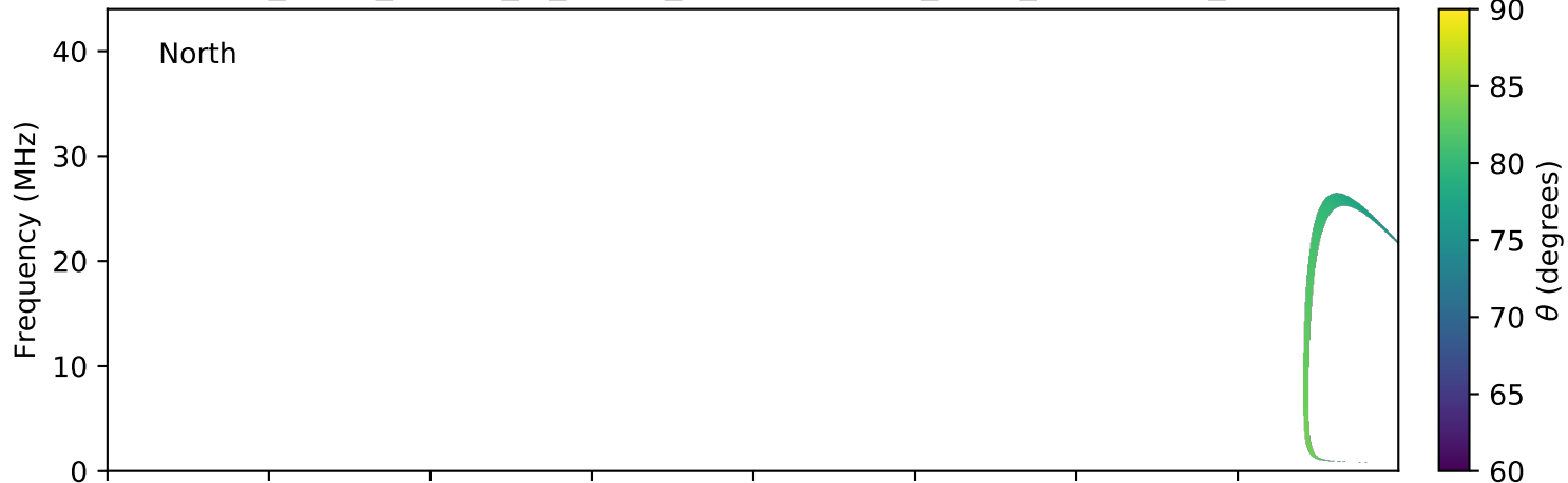
expres_earth_jupiter_io_jrm09_lossc-wid1deg_3kev_20130408_v01.cdf
