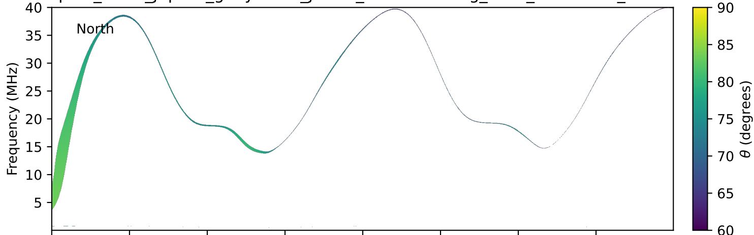
expres_earth_jupiter_ganymede_jrm33_lossc-wid1deg_3kev_20130427_v11.cdf
