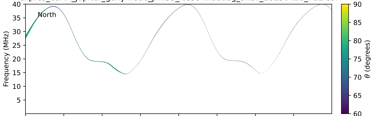
expres_earth_jupiter_ganymede_jrm33_lossc-wid1deg_3kev_20130420_v11.cdf
