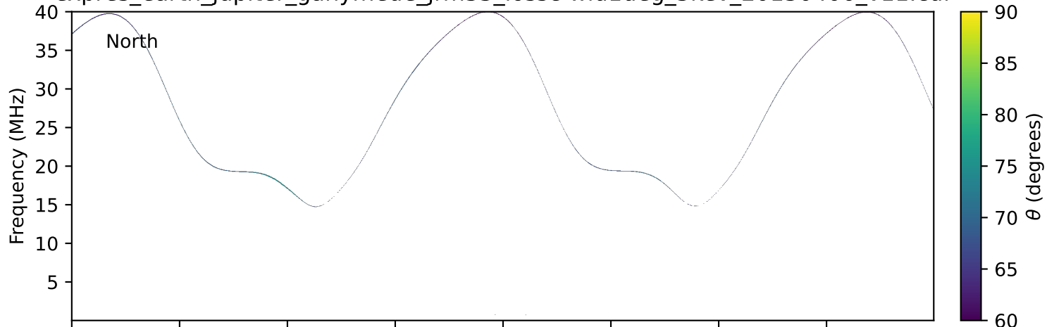
expres_earth_jupiter_ganymede_jrm33_lossc-wid1deg_3kev_20130406_v11.cdf
