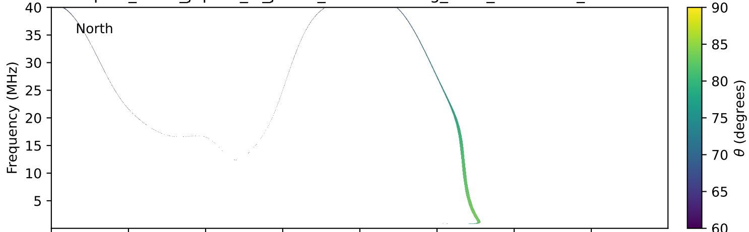
expres_earth_jupiter_io_jrm33_lossc-wid1deg_3kev_20130222_v11.cdf
