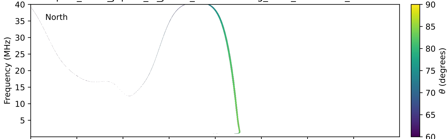
expres_earth_jupiter_io_jrm33_lossc-wid1deg_3kev_20130208_v11.cdf
