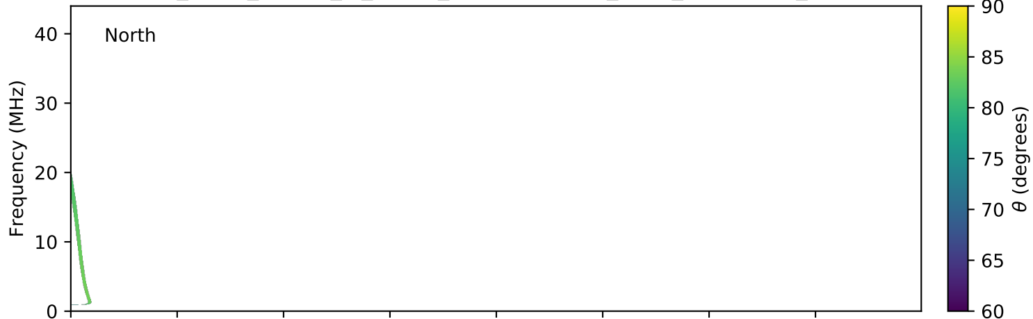
expres_earth_jupiter_io_jrm09_lossc-wid1deg_3kev_20130228_v01.cdf
