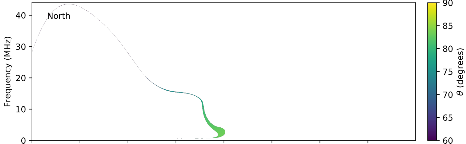
expres_earth_jupiter_io_jrm09_lossc-wid1deg_3kev_20130224_v01.cdf
