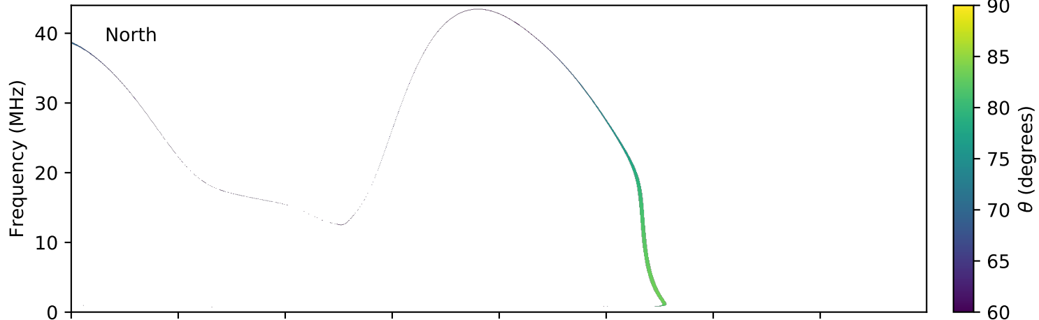
expres_earth_jupiter_io_jrm09_lossc-wid1deg_3kev_20130222_v01.cdf
