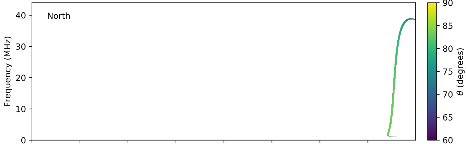
expres_earth_jupiter_io_jrm09_lossc-wid1deg_3kev_20130221_v01.cdf
