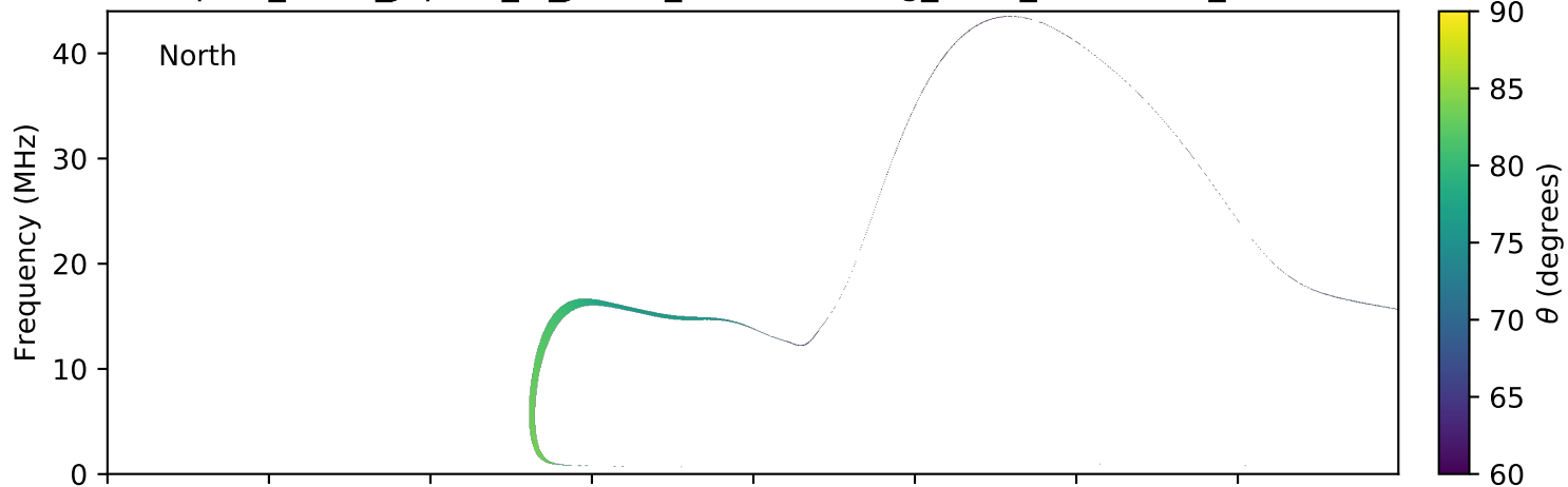
expres_earth_jupiter_io_jrm09_lossc-wid1deg_3kev_20130218_v01.cdf
