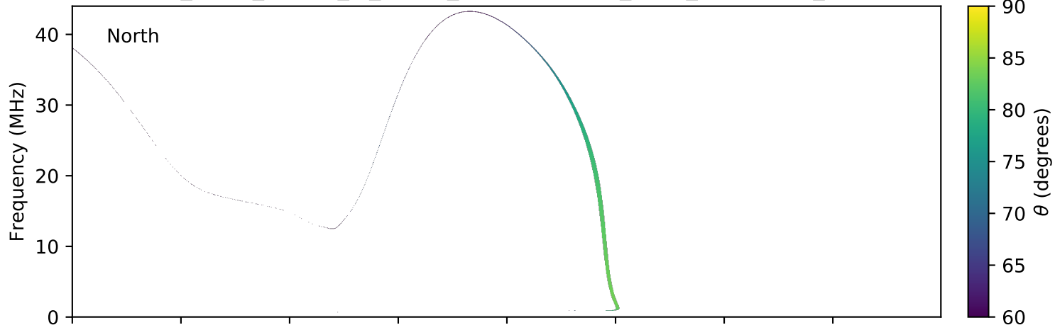
expres_earth_jupiter_io_jrm09_lossc-wid1deg_3kev_20130215_v01.cdf
