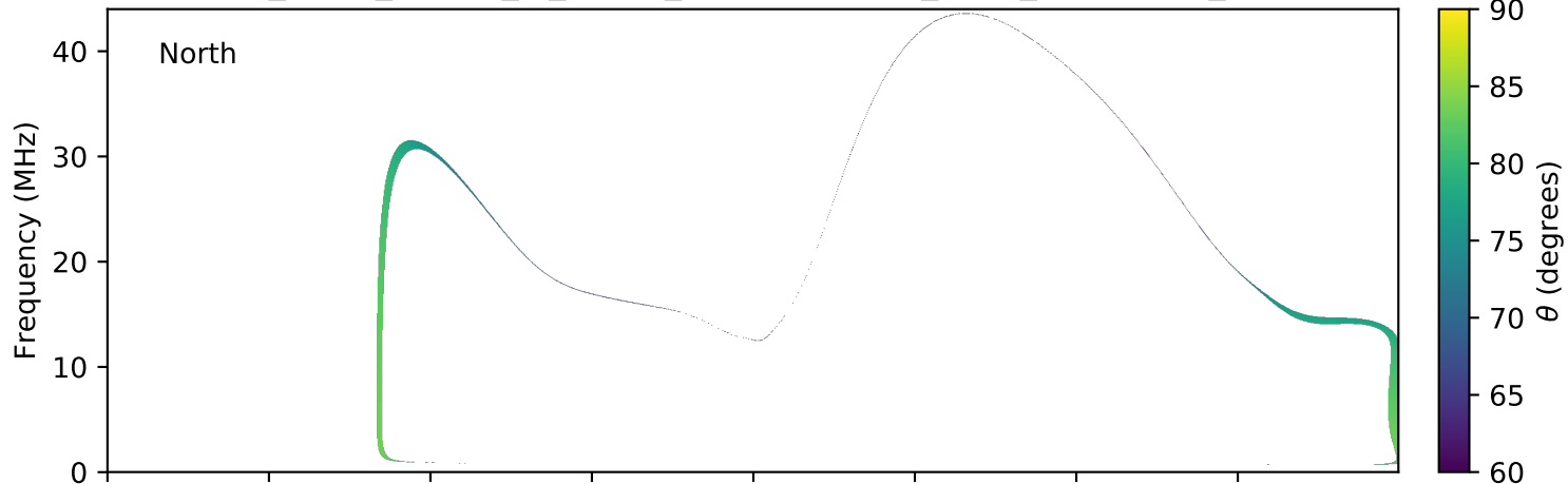
expres_earth_jupiter_io_jrm09_lossc-wid1deg_3kev_20130204_v01.cdf
