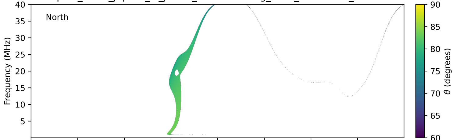
expres_earth_jupiter_io_jrm33_lossc-wid1deg_3kev_20130126_v11.cdf
