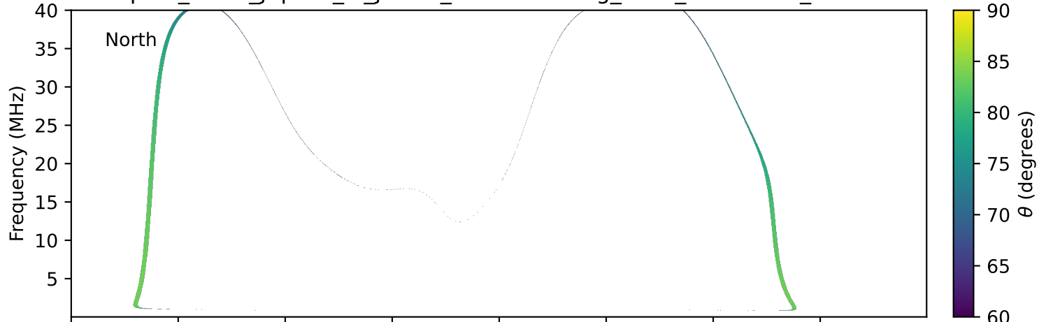
expres_earth_jupiter_io_jrm33_lossc-wid1deg_3kev_20130121_v11.cdf
