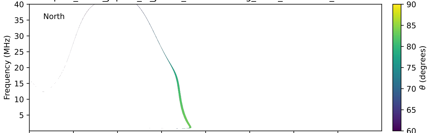
expres_earth_jupiter_io_jrm33_lossc-wid1deg_3kev_20130109_v11.cdf
