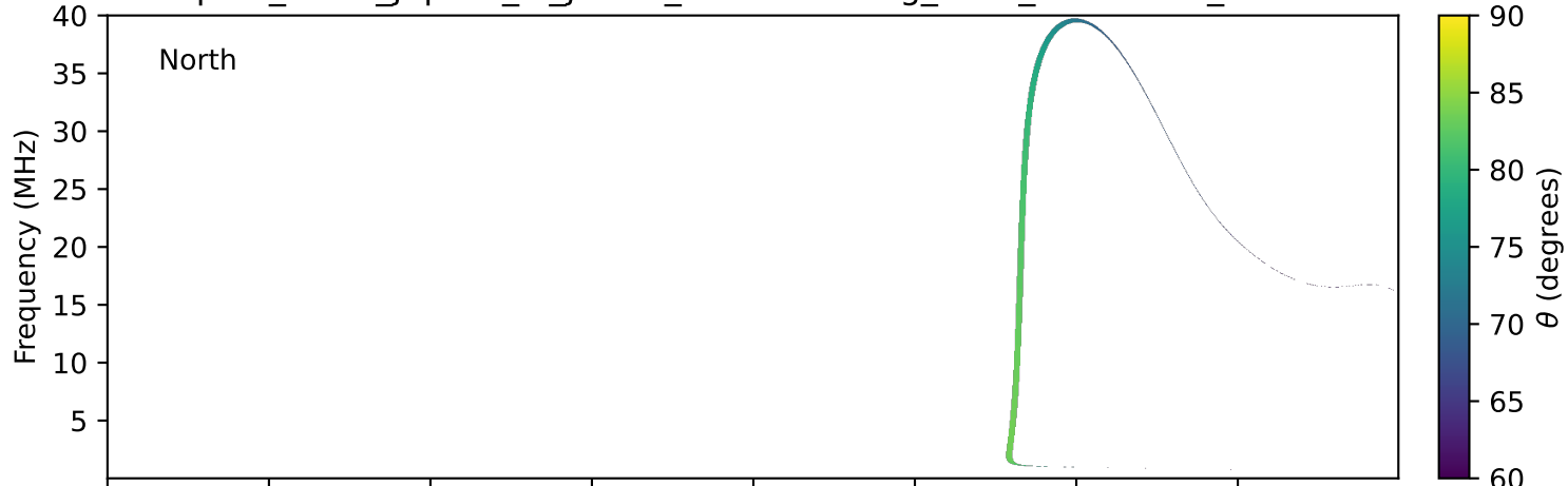
expres_earth_jupiter_io_jrm33_lossc-wid1deg_3kev_20130108_v11.cdf
