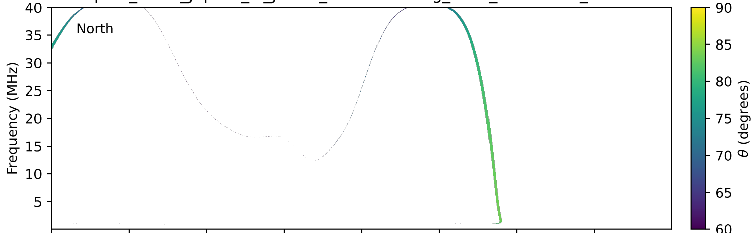
expres_earth_jupiter_io_jrm33_lossc-wid1deg_3kev_20130107_v11.cdf
