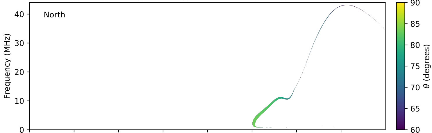
expres_earth_jupiter_io_jrm09_lossc-wid1deg_3kev_20130131_v01.cdf
