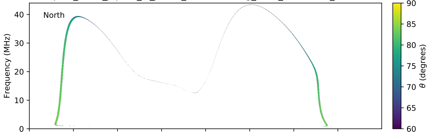
expres_earth_jupiter_io_jrm09_lossc-wid1deg_3kev_20130121_v01.cdf
