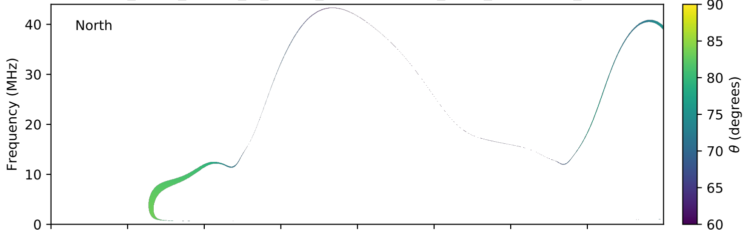
expres_earth_jupiter_io_jrm09_lossc-wid1deg_3kev_20130112_v01.cdf
