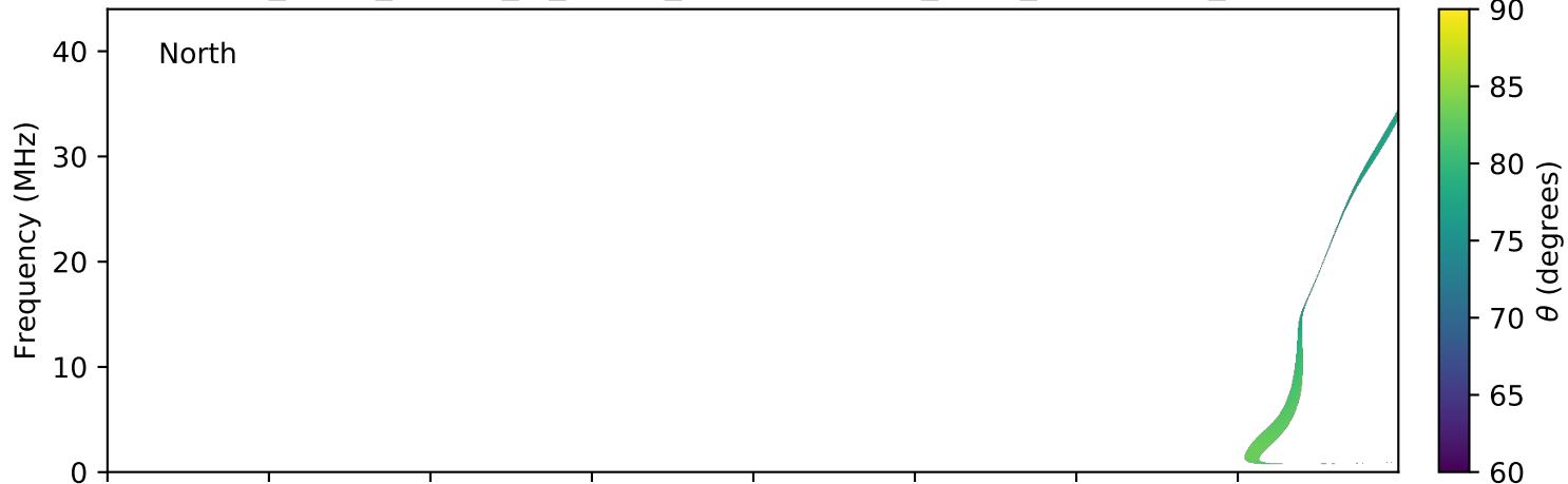
expres_earth_jupiter_io_jrm09_lossc-wid1deg_3kev_20130106_v01.cdf
