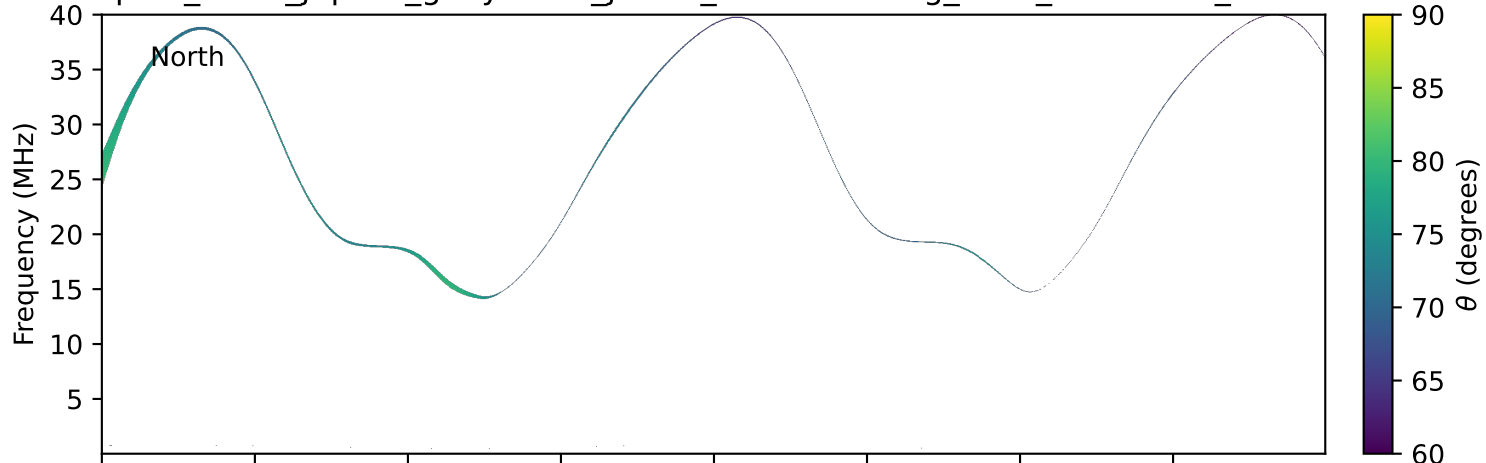
expres_earth_jupiter_ganymede_jrm33_lossc-wid1deg_3kev_20130131_v11.cdf
