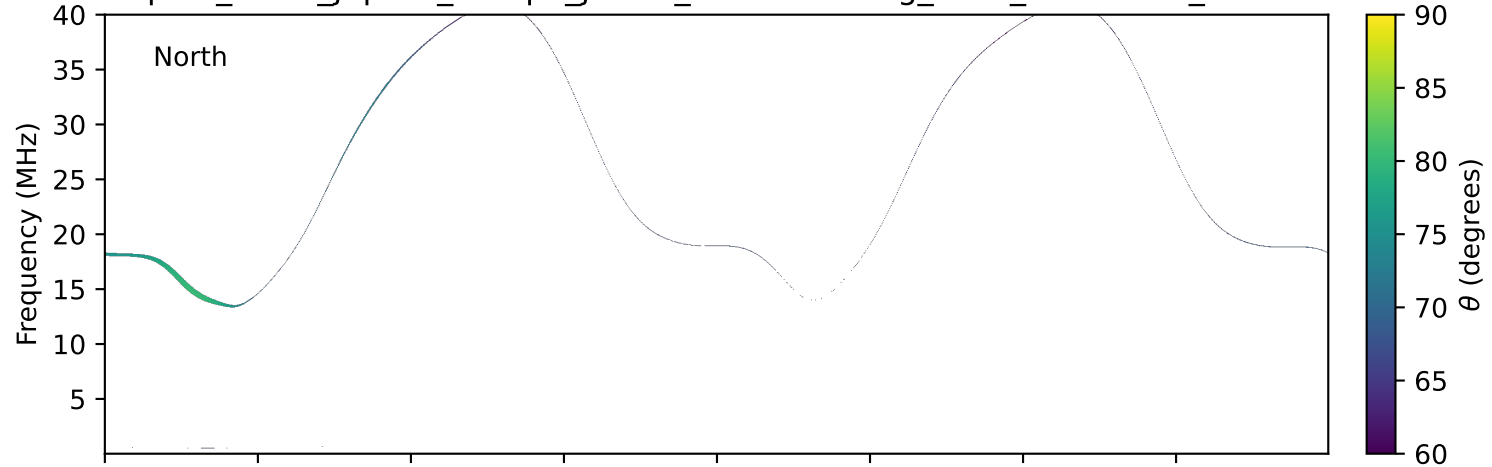
expres_earth_jupiter_europa_jrm33_lossc-wid1deg_3kev_20130125_v11.cdf
