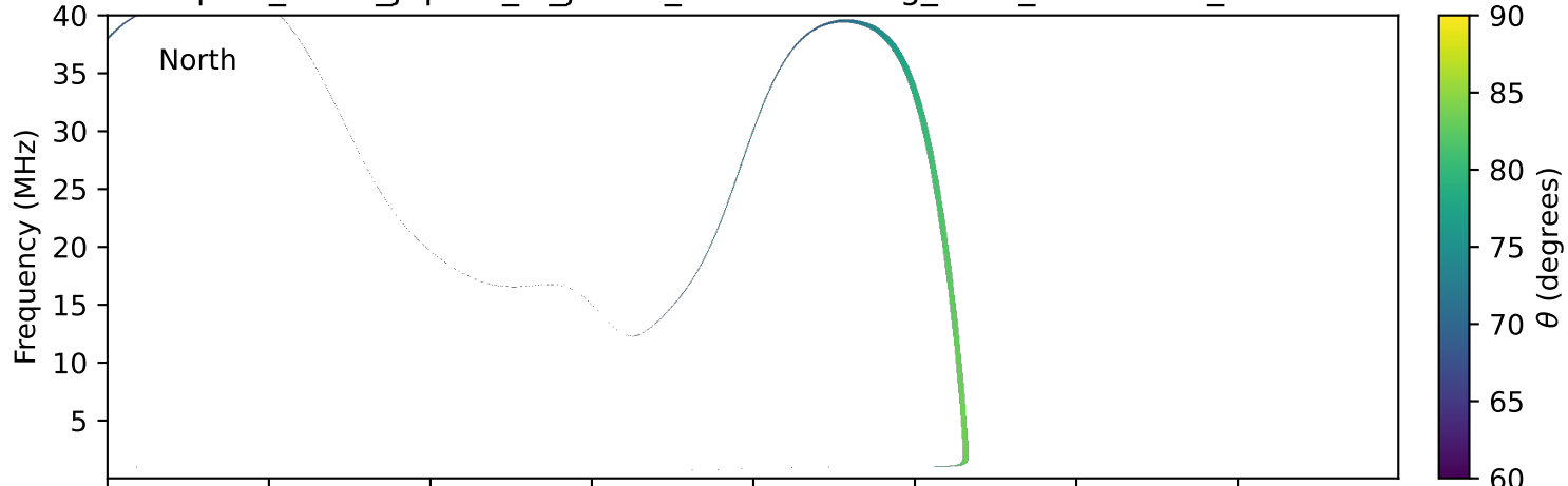
expres_earth_jupiter_io_jrm33_lossc-wid1deg_3kev_20121231_v11.cdf
