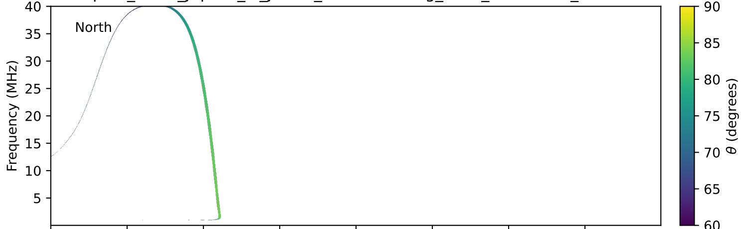
expres_earth_jupiter_io_jrm33_lossc-wid1deg_3kev_20121219_v11.cdf
