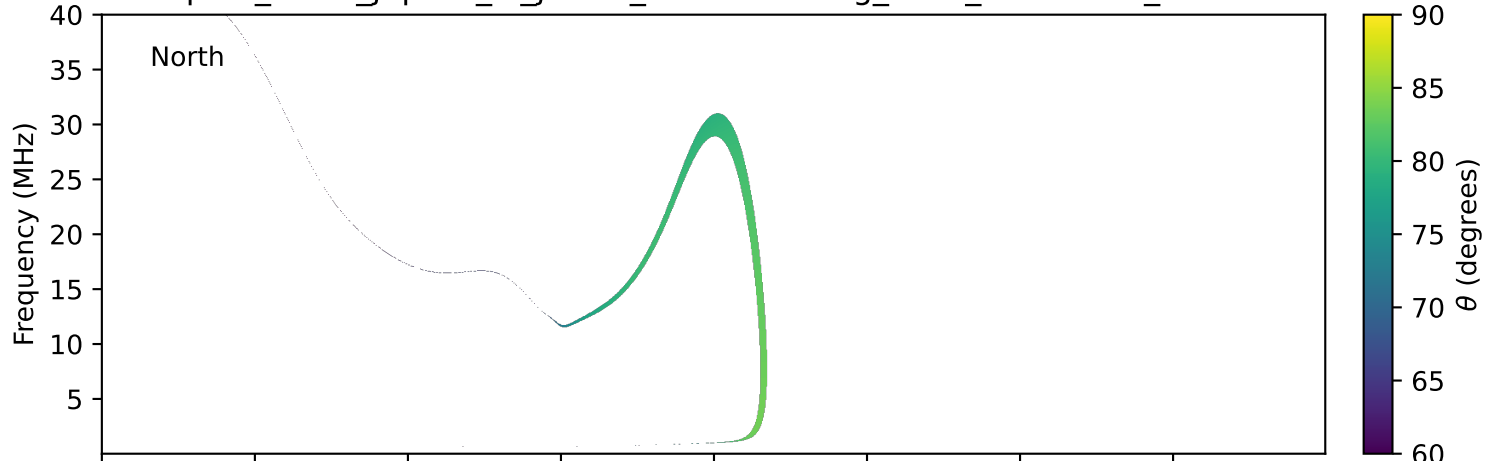
expres_earth_jupiter_io_jrm33_lossc-wid1deg_3kev_20121217_v11.cdf
