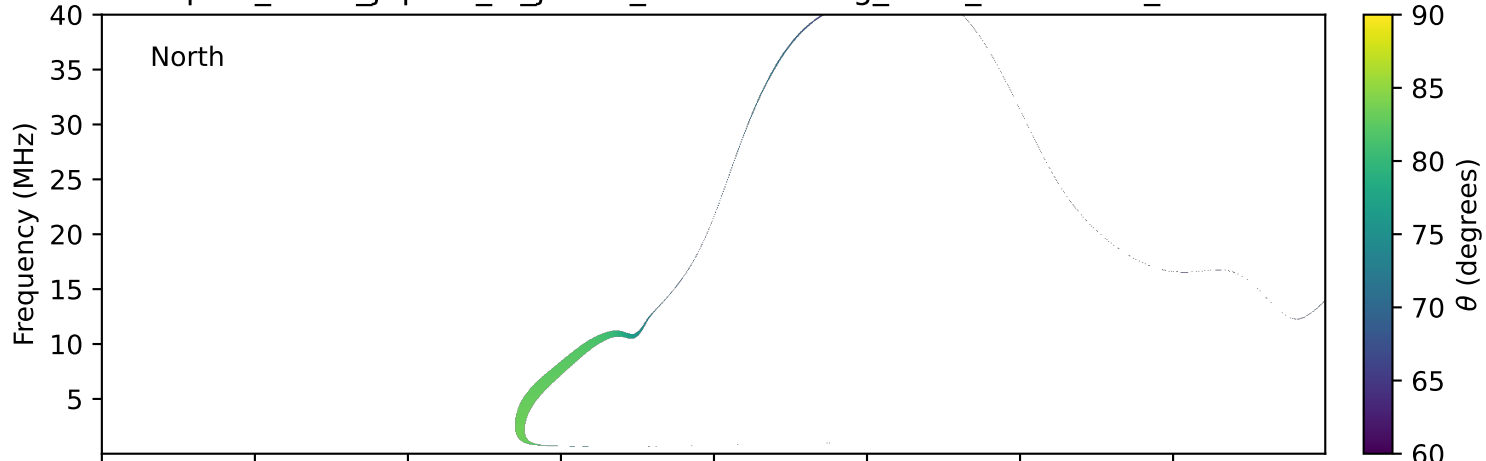
expres_earth_jupiter_io_jrm33_lossc-wid1deg_3kev_20121211_v11.cdf
