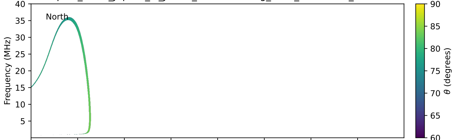
expres_earth_jupiter_io_jrm33_lossc-wid1deg_3kev_20121205_v11.cdf
