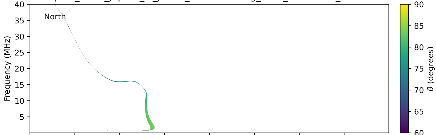
expres_earth_jupiter_io_jrm33_lossc-wid1deg_3kev_20121203_v11.cdf
